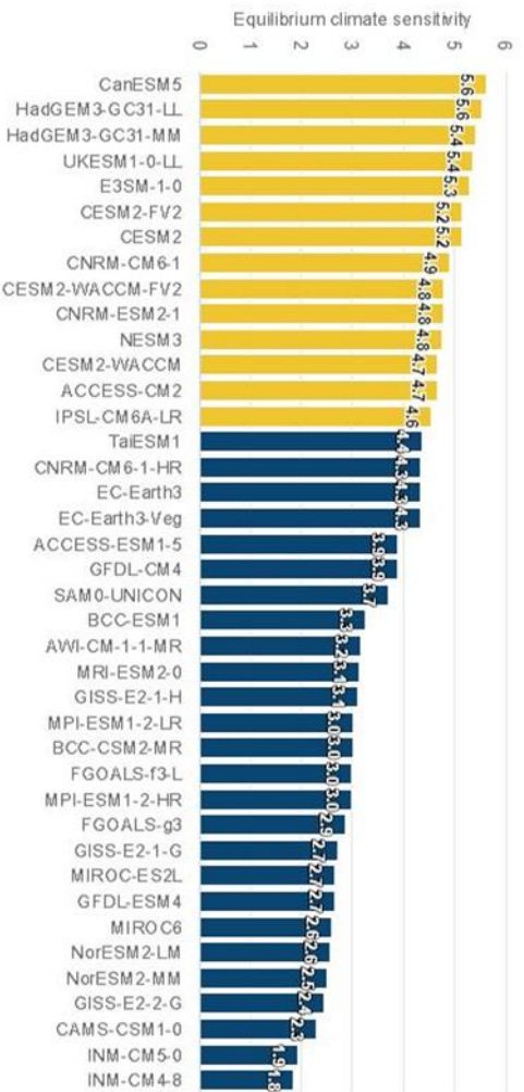
Figure 4. The CMIP6 model suite. Models warmer than the warmest CMIP5 versions are in yellow. The models with the lowest ECS are the Russian INM-CM4.8 (1.8°C) and INM-CM5.0 (1.9°C). In CMIP5, the INM-CM4 ECS was 2.05°C. Those three models conform to observed temperatures better than the others.
