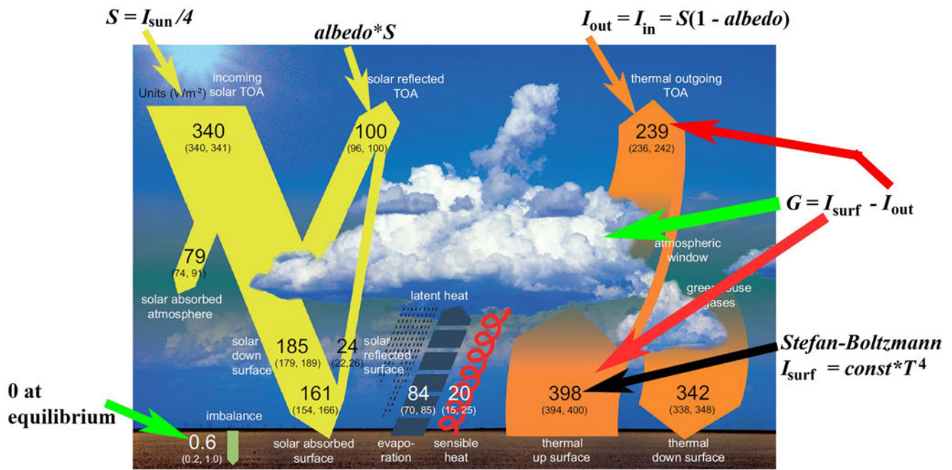
Figure 3: The heat-flow drawing from AR5, showing how the drawing comports with Eq. 4.
