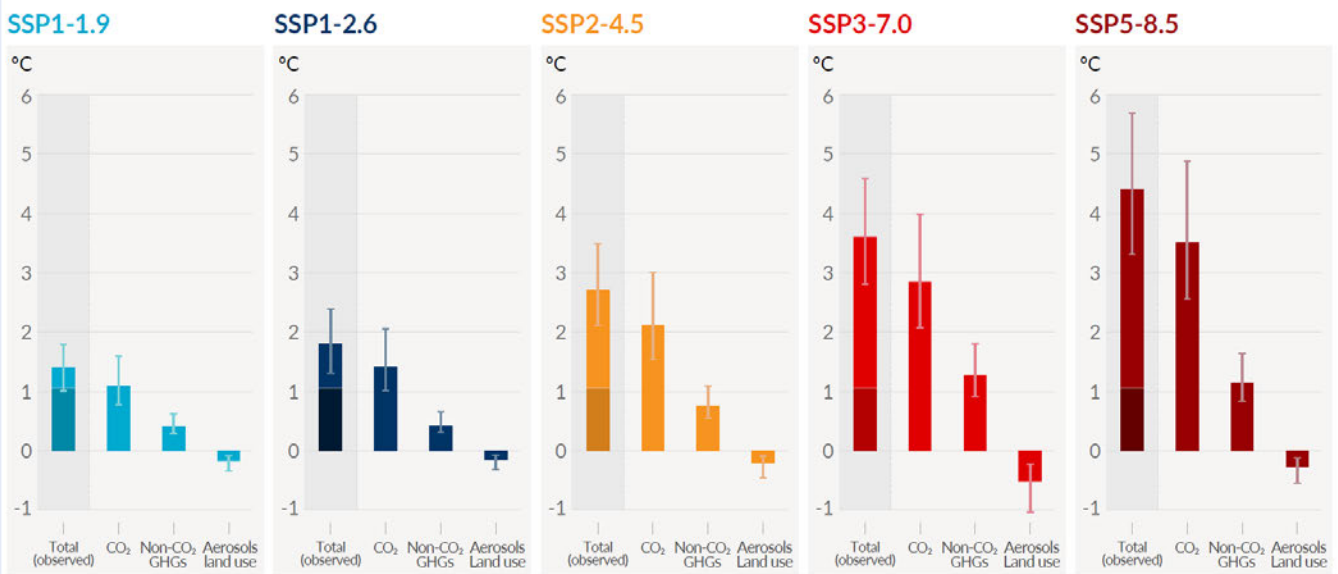
Figure 5: Five scenarios from the Summary for Policy Makers in the Sixth Assessment Report (AR6) in 2021.
