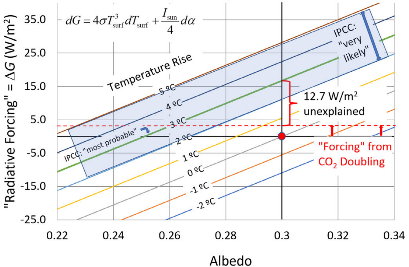
Figure 4: The differential form of the climate constraint equation. The red dot shows the current situation. The dashed red line shows the “radiative forcing” ( =3.47 \text{ W/m}^2 , IPCC) due to doubling \text{CO}_2 concentration, and the green slanted line shows IPCC’s “most probable” temperature rise of 3^\circ\text{C} . IPCC says that the rise due to doubling is “very likely” to be between 2^\circ\text{C} and 5^\circ\text{C} . A temperature rise dT_{\text{surf}} of 3^\circ\text{C} will increase surface radiation by 16.5 \text{ W/m}^2 . IPCC has no explanation and no description of how 3.47 \text{ W/m}^2 can cause 16.5 \text{ W/m}^2 of increased surface radiation.
